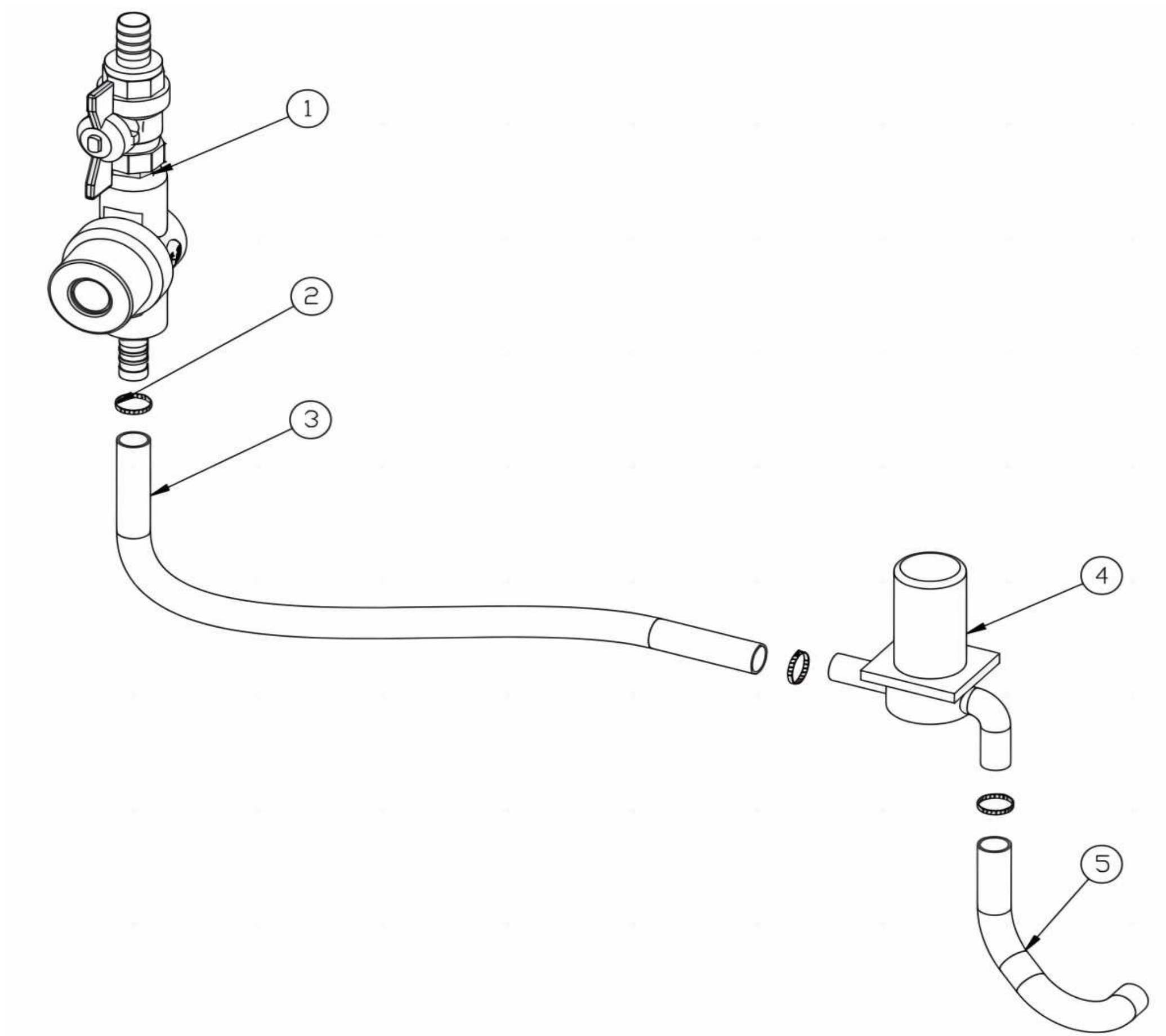
Fig. 6 -HOSE GROUP
