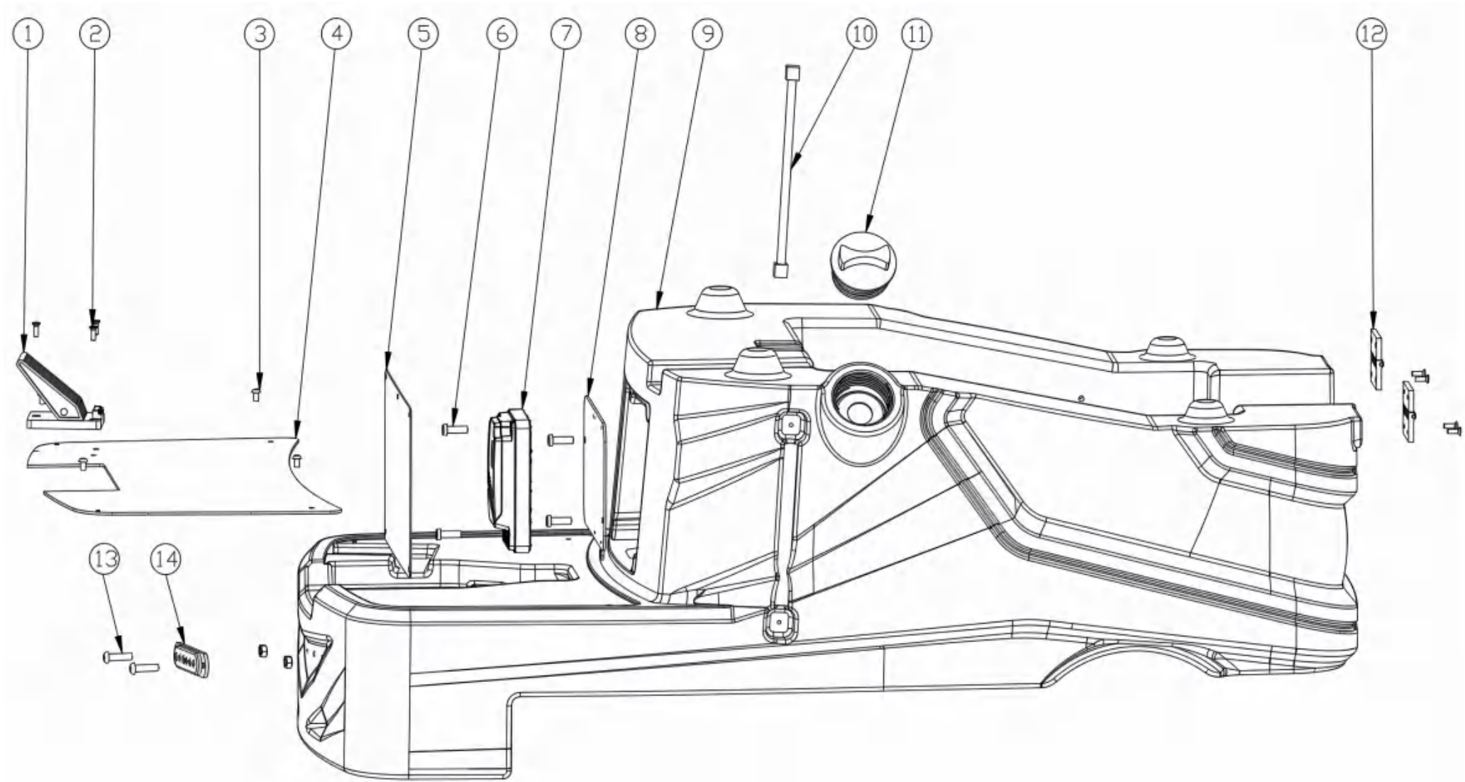
Fig. 2 -SOLUTION TANK GROUP
